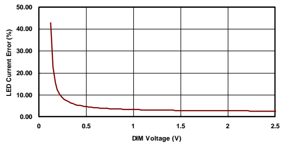
Dimming Voltage VS LED Current Error
