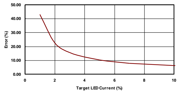
Target LED Current VS LED Current Error(ZOOM IN)
